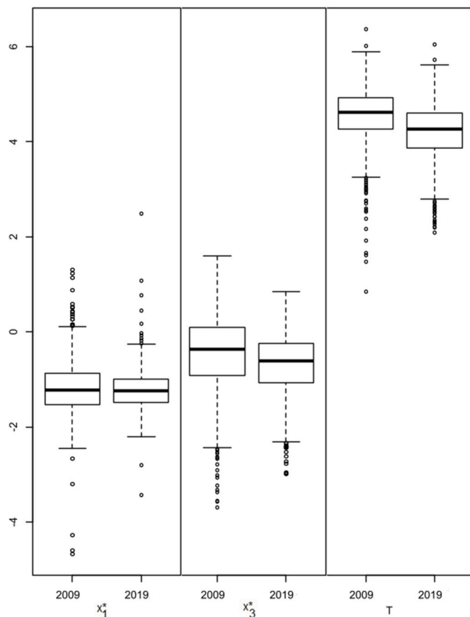
Fig. 5. Boxplots of the balance coordinates x^*_1 , x^*_3 and the total by 2009 and 2019.
