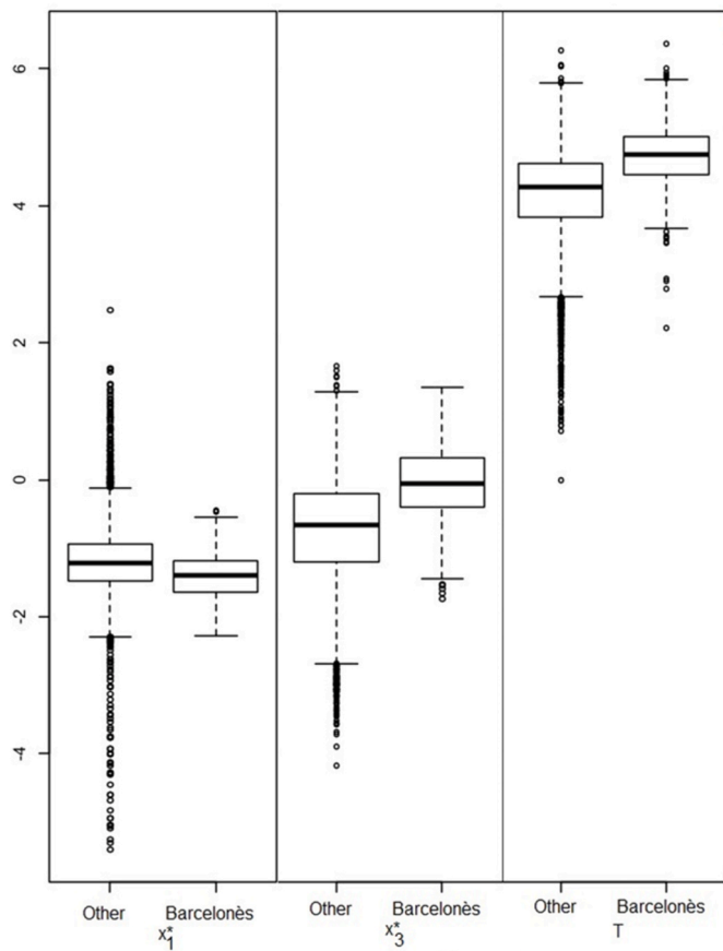
Fig. 3. Boxplots of the balance coordinates x^*_1 , x^*_3 and the total by location (Barcelonès versus other areas) during the period 2009–2019.
