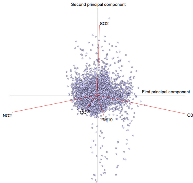
Fig. 2. Compositional covariance biplot.
