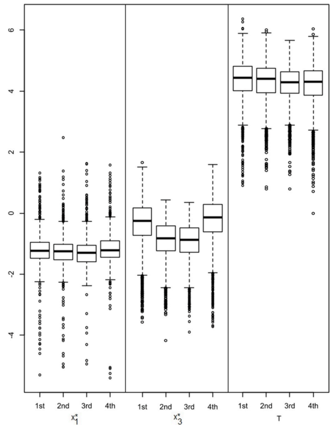
Fig. 4. Boxplots of the balance coordinates x^*_1 , x^*_3 and the total by quarters during the period 2009–2019. Note: First quarter: January to March; Second quarter: April to June; Third quarter: July to September; Fourth quarter: October to December.
