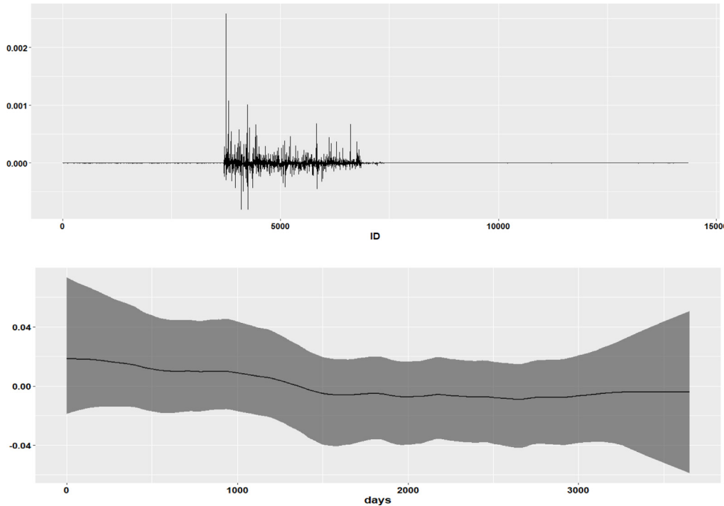
Fig. A.11. Top: Marginal posterior mean of the spatial random effect S(\cdot) . Bottom: Marginal posterior mean of the temporal random effect \delta_{\tau} .
