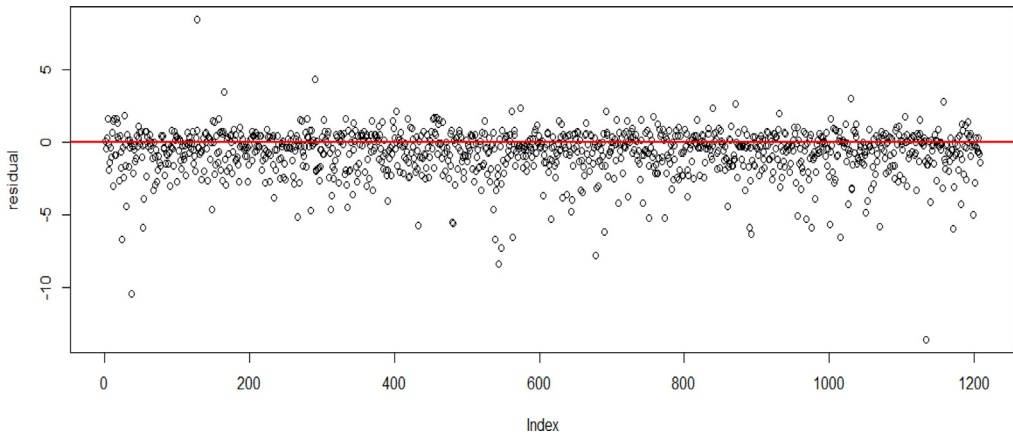
Fig. 5. Residual (observed minus predicted) plots.
